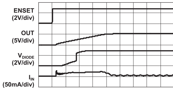
Time (100µs/div)
